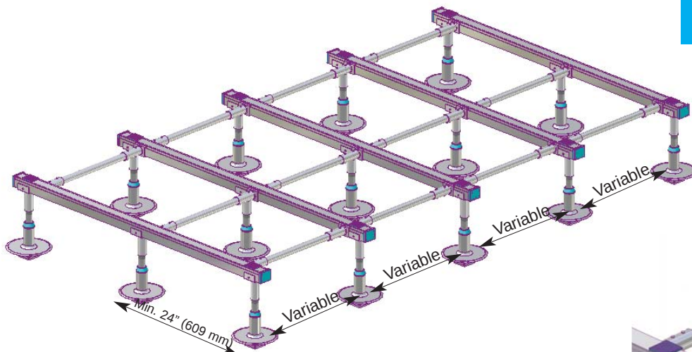
MERS-920A ALUMINUM AIR HANDLING UNIT SUPPORT (Large Unit)
