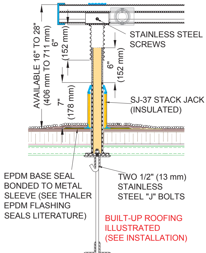
TYPICAL MERS-900 ALUMINUM A/C UNIT SUPPORT (LARGE SCALE DETAIL)
