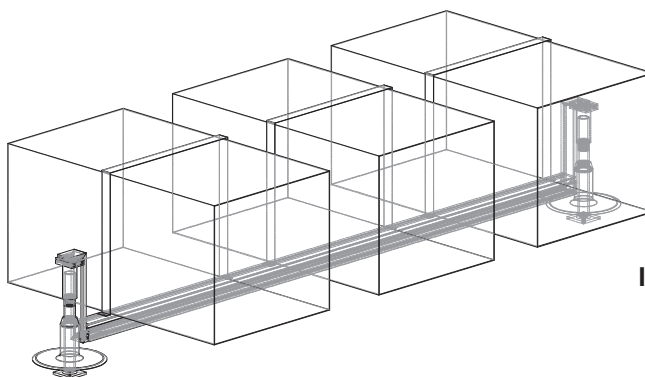
MERS-850A RE-ROOFING MULTIPLE DUCT SUPPORT
