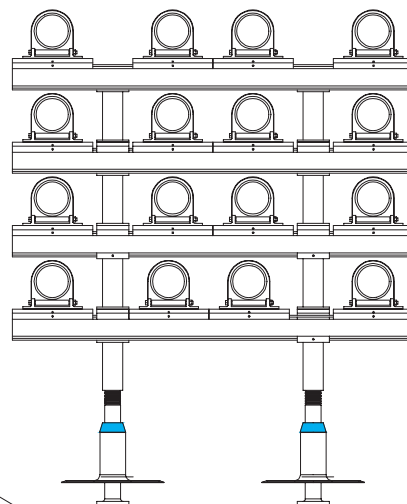
END VIEW
